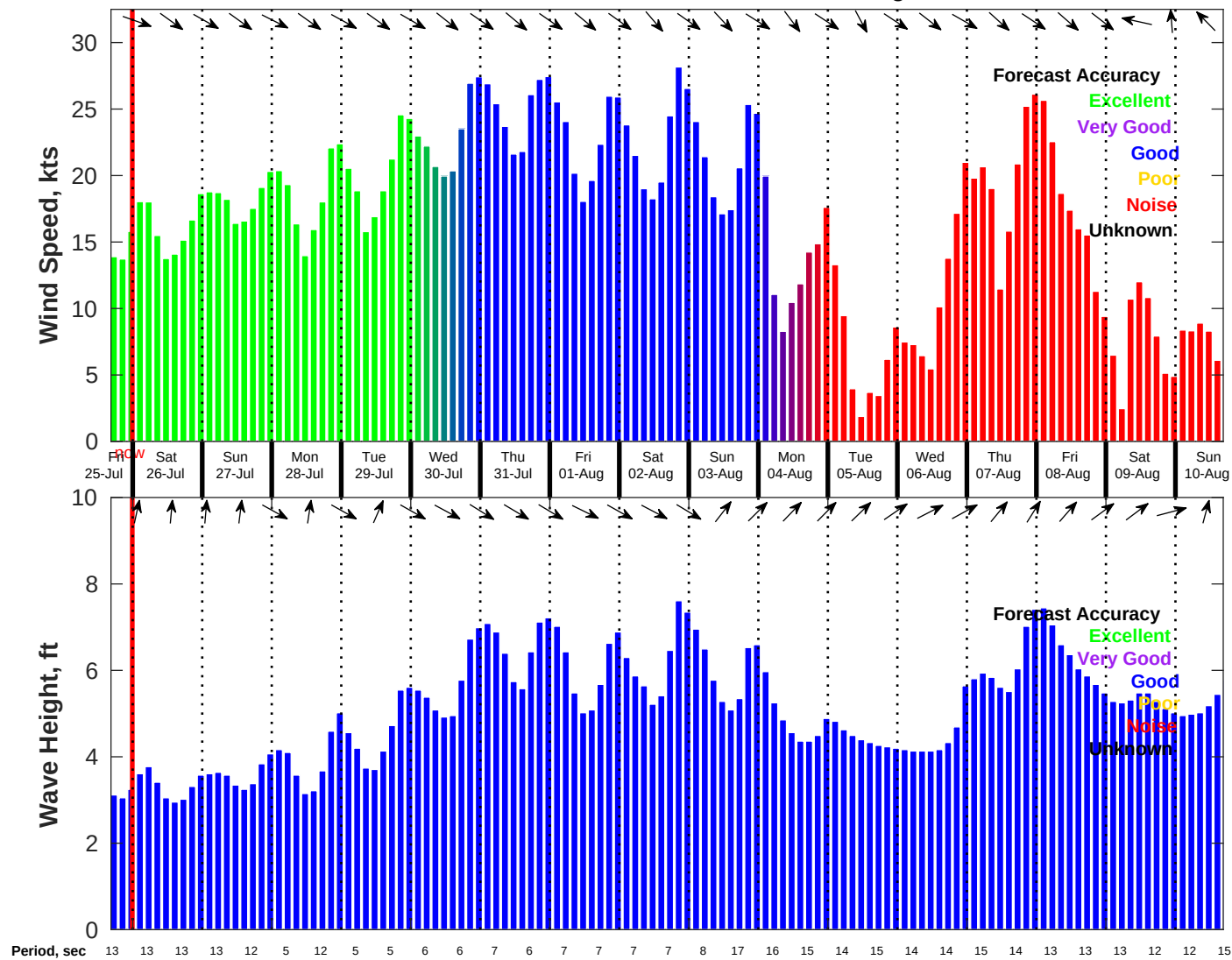
Wind & Wave Forecast for NDBC 46069 from 25-Jul-2025 16:00:00 to 10-Aug-2025 16:00:00
