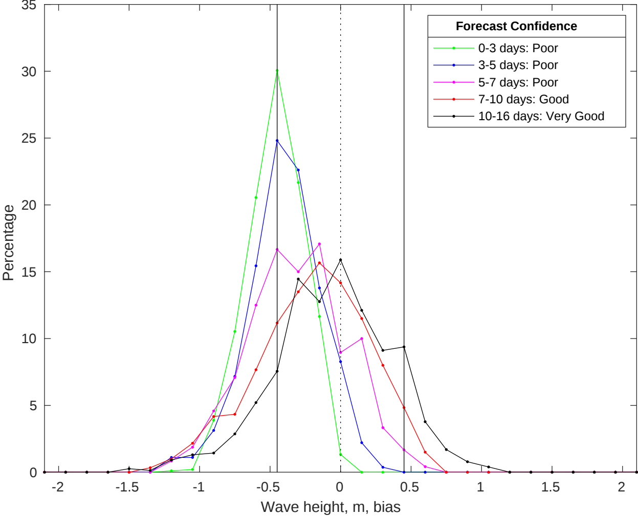
NDBC 51209 vs GFS Waves Bias Histogram: 26-Jul-2025
