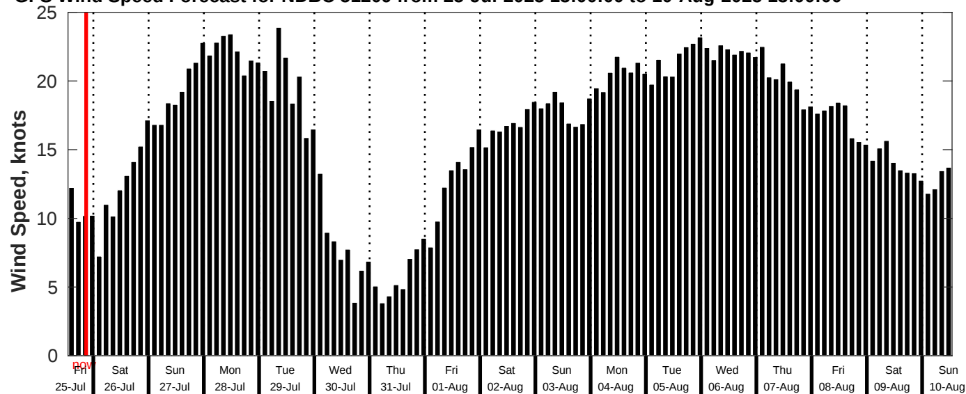
GFS Wind Speed Forecast for NDBC 51209 from 25-Jul-2025 13:00:00 to 10-Aug-2025 13:00:00
