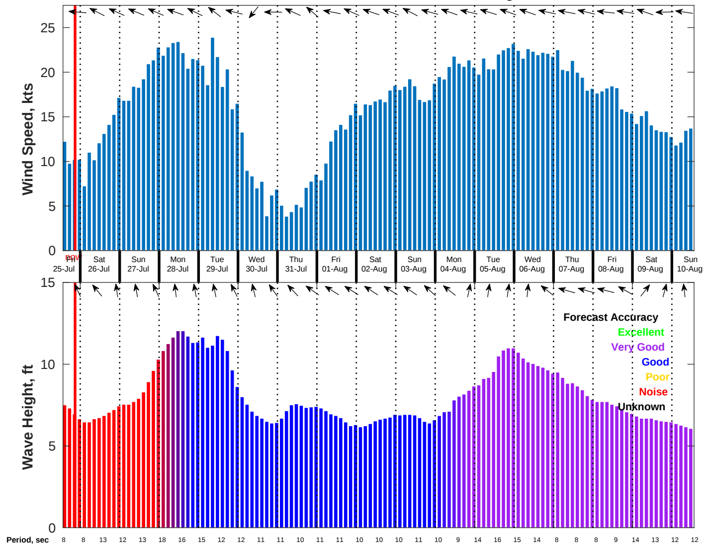
Wind & Wave Forecast for NDBC 51209 from 25-Jul-2025 13:00:00 to 10-Aug-2025 13:00:00
