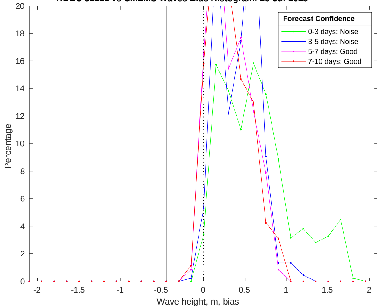
NDBC 51211 vs CMEMS Waves Bias Histogram: 26-Jul-2025
