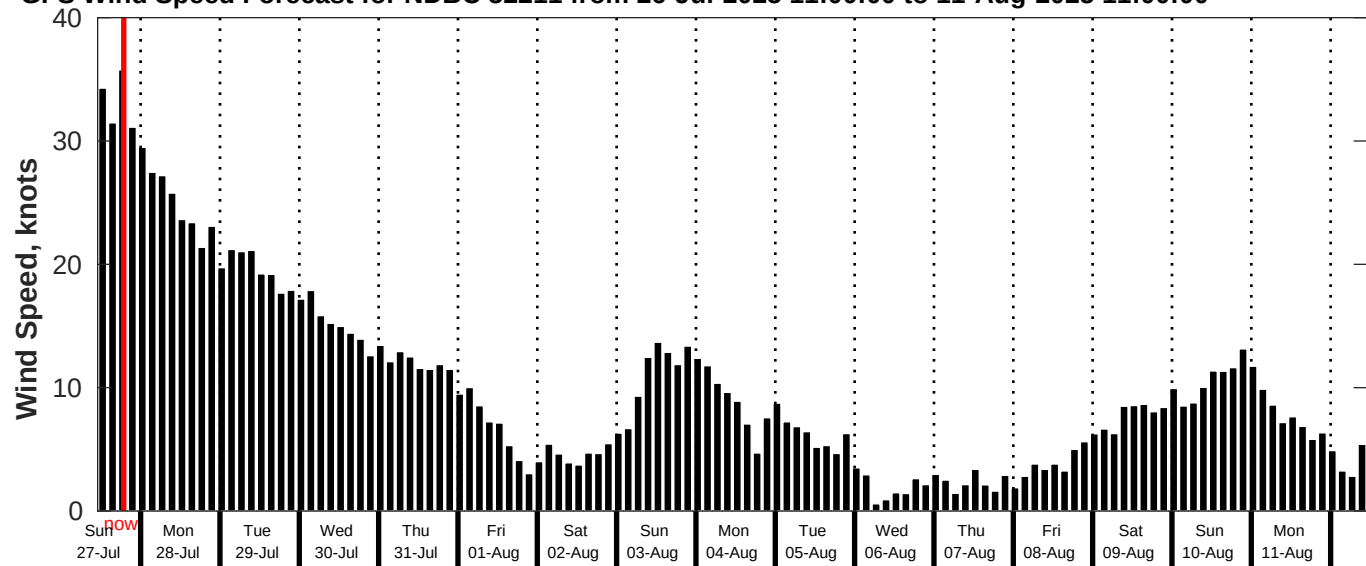
GFS Wind Speed Forecast for NDBC 52211 from 26-Jul-2025 11:00:00 to 11-Aug-2025 11:00:00
