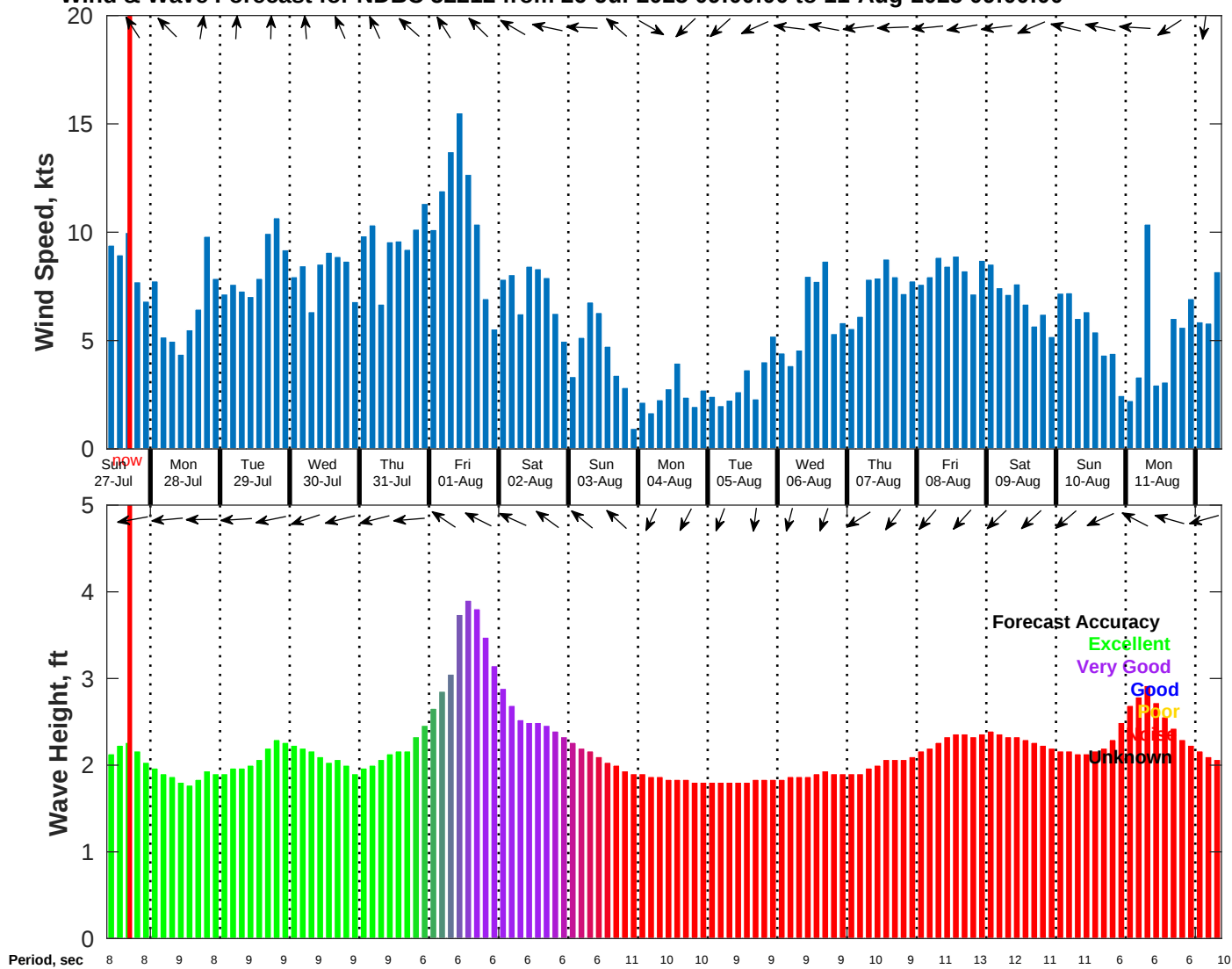
Wind & Wave Forecast for NDBC 52212 from 26-Jul-2025 09:00:00 to 11-Aug-2025 09:00:00
