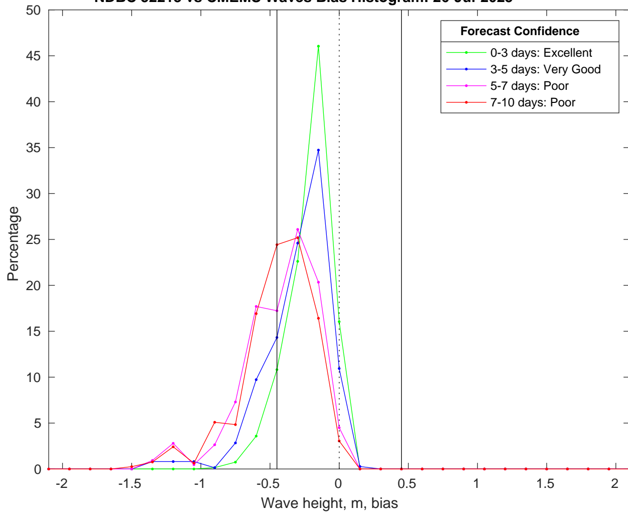
NDBC 52213 vs CMEMS Waves Bias Histogram: 26-Jul-2025
