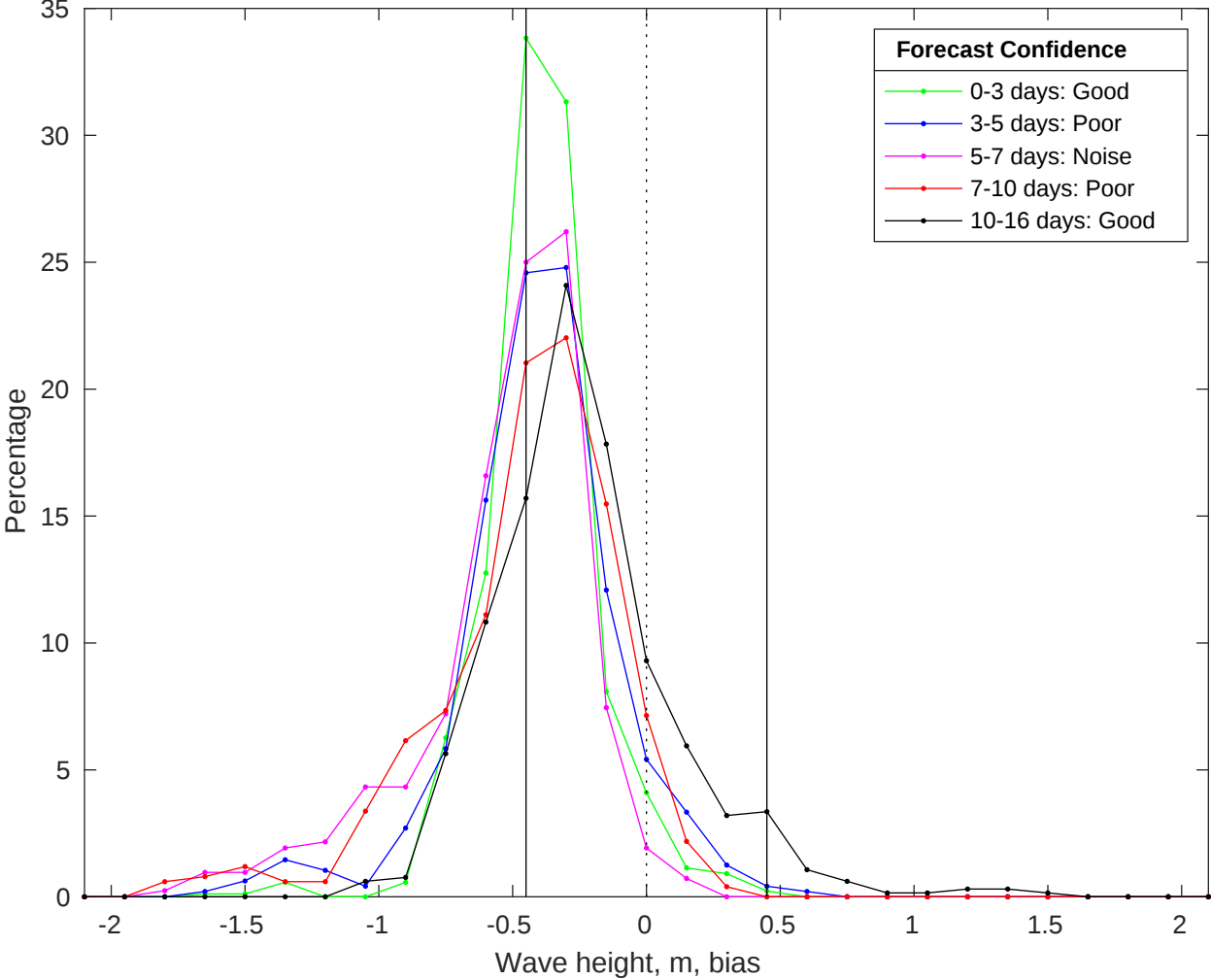
NDBC 52213 vs GFS Waves Bias Histogram: 26-Jul-2025
