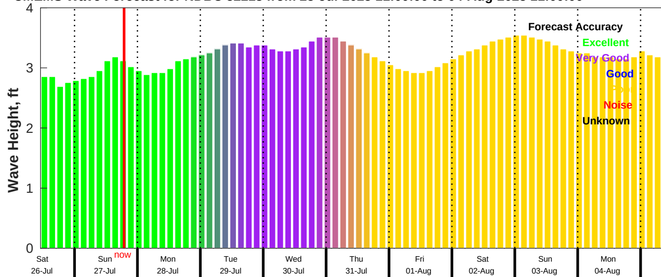
CMEMS Wave Forecast for NDBC 52213 from 25-Jul-2025 11:00:00 to 04-Aug-2025 11:00:00
