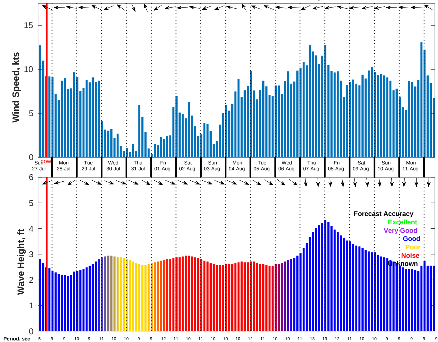
Wind & Wave Forecast for NDBC 52213 from 26-Jul-2025 11:00:00 to 11-Aug-2025 11:00:00
