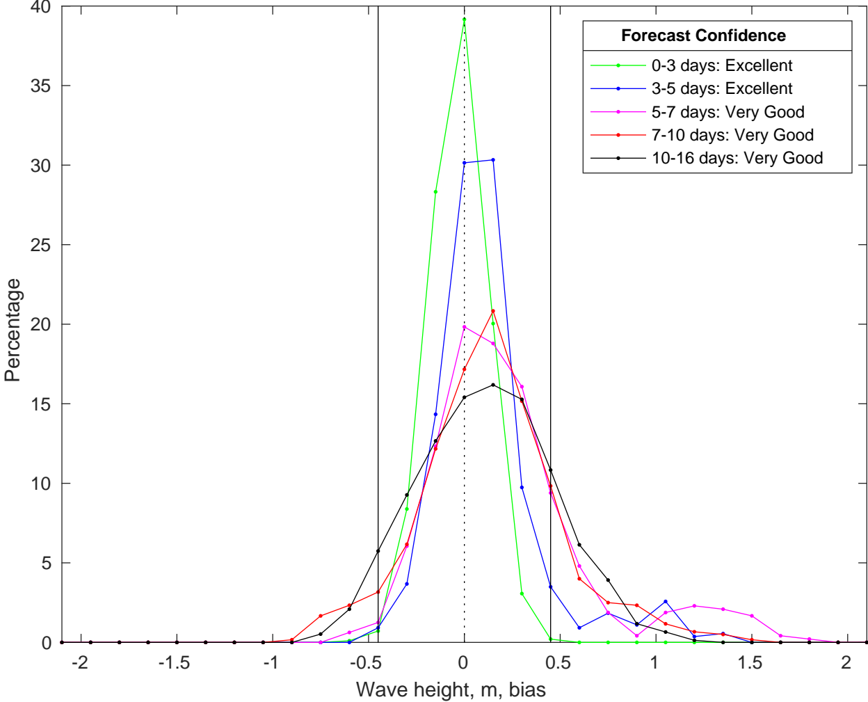
NDBC 41004 vs GFS Waves Bias Histogram: 27-Jul-2025
