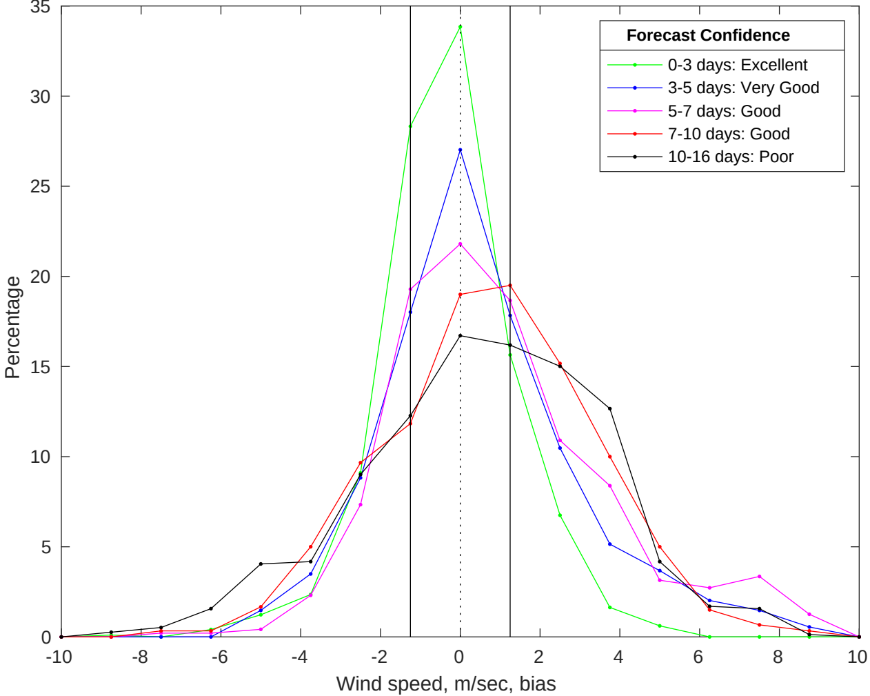
NDBC 41004 vs GFS Winds Bias Histogram: 27-Jul-2025
