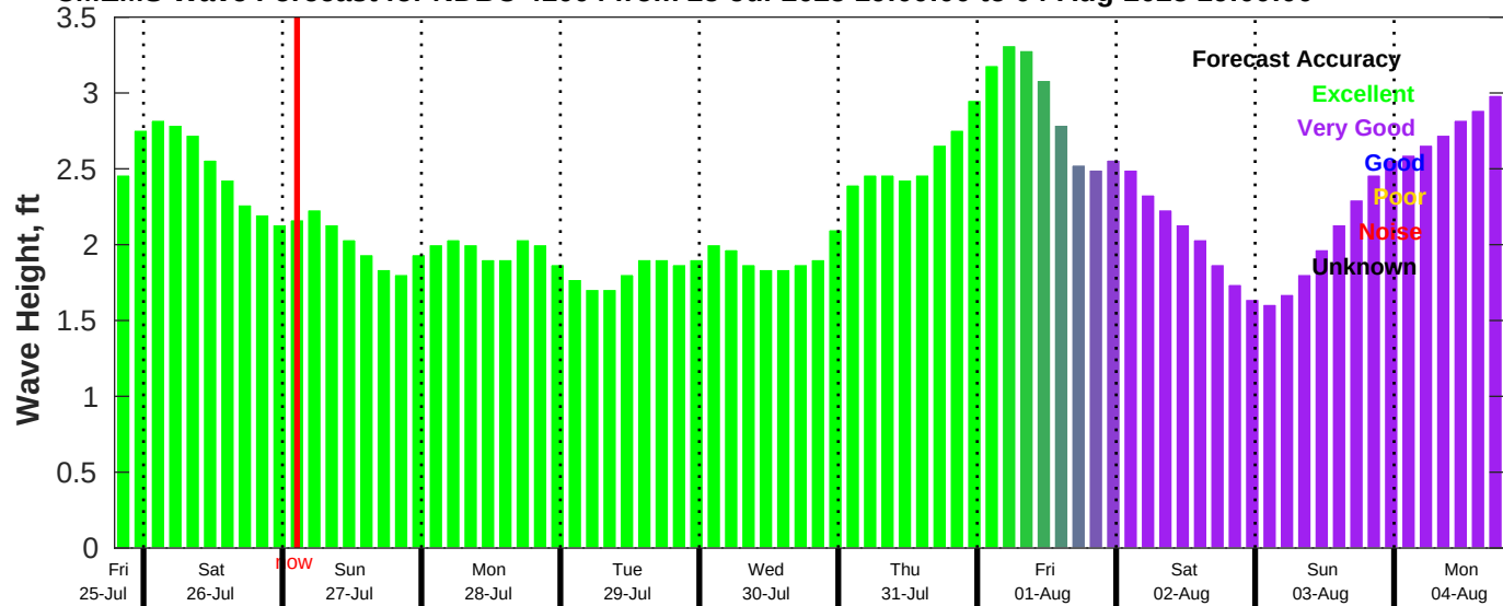
CMEMS Wave Forecast for NDBC 41004 from 25-Jul-2025 19:00:00 to 04-Aug-2025 19:00:00
