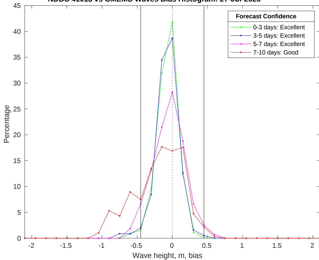
NDBC 41013 vs CMEMS Waves Bias Histogram: 27-Jul-2025
