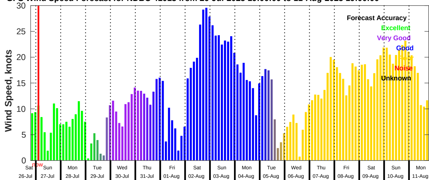
GFS Wind Speed Forecast for NDBC 41013 from 26-Jul-2025 19:00:00 to 11-Aug-2025 19:00:00
