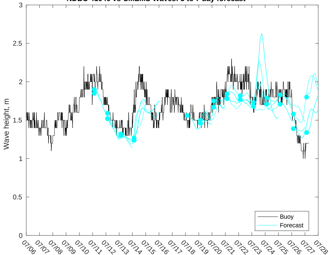
NDBC 41040 vs CMEMS Waves: 5 to 7 day forecast
