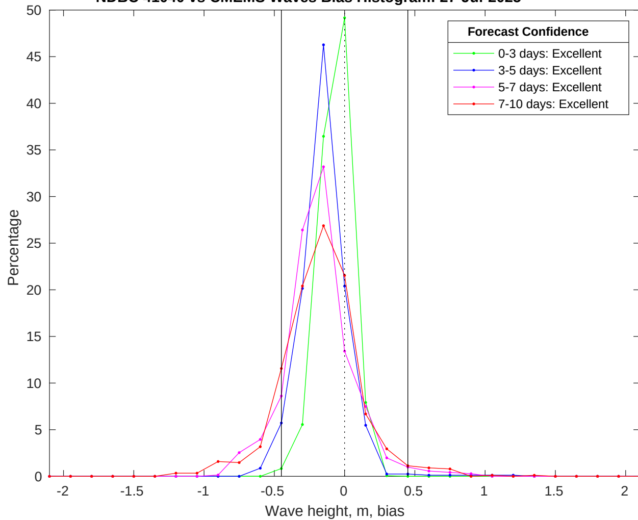
NDBC 41040 vs CMEMS Waves Bias Histogram: 27-Jul-2025
