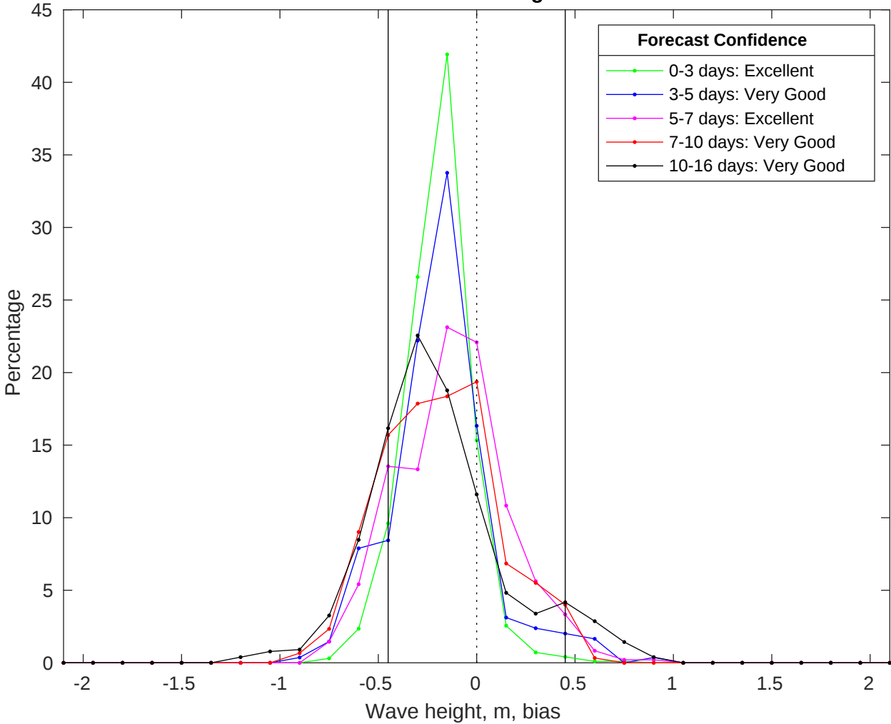
NDBC 41040 vs GFS Waves Bias Histogram: 27-Jul-2025
