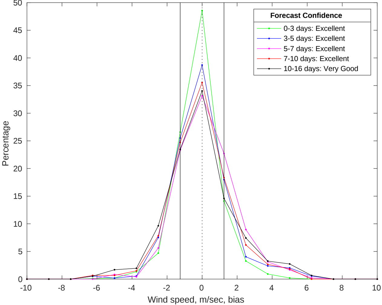
NDBC 41040 vs GFS Winds Bias Histogram: 27-Jul-2025
