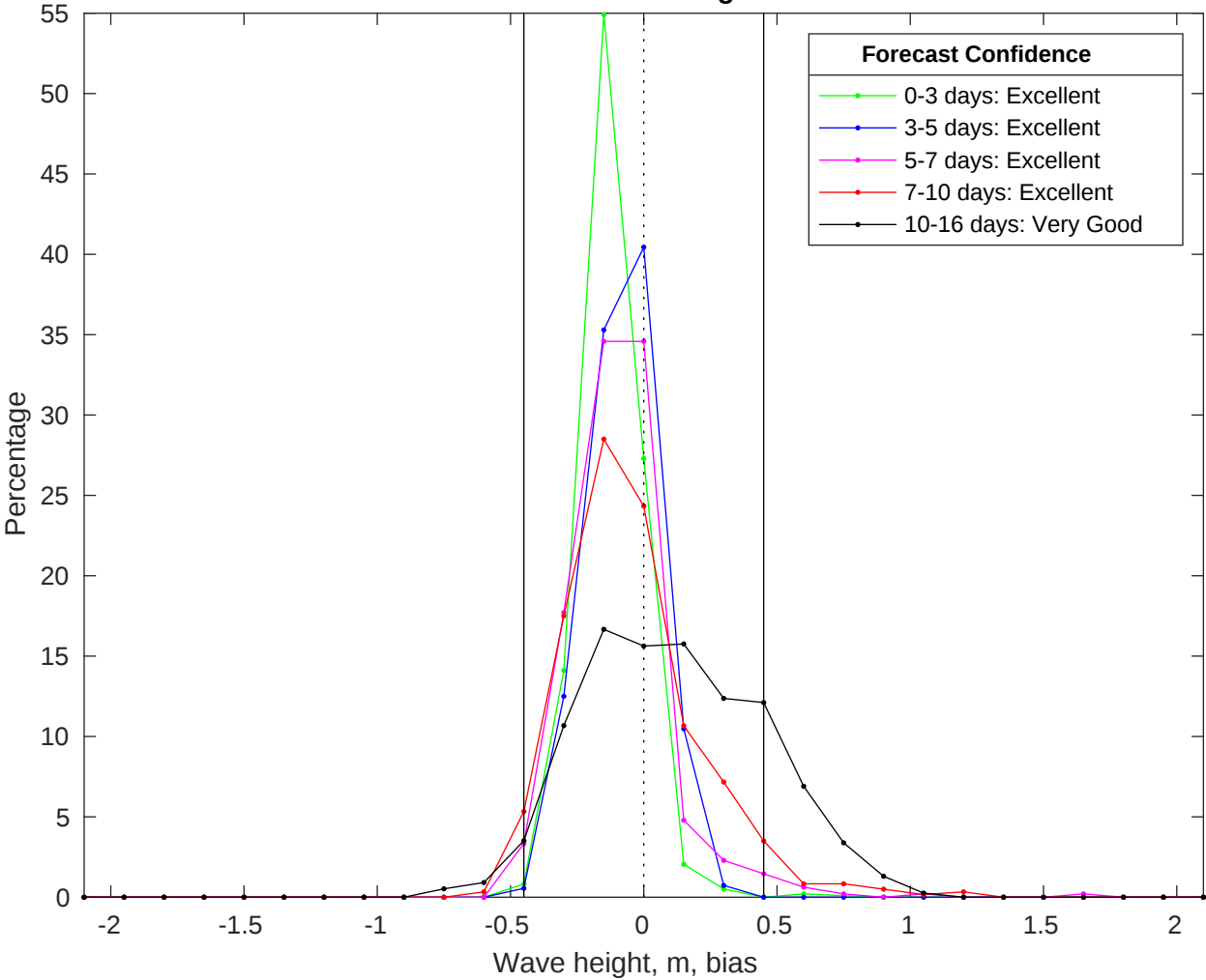
NDBC 42019 vs GFS Waves Bias Histogram: 27-Jul-2025
