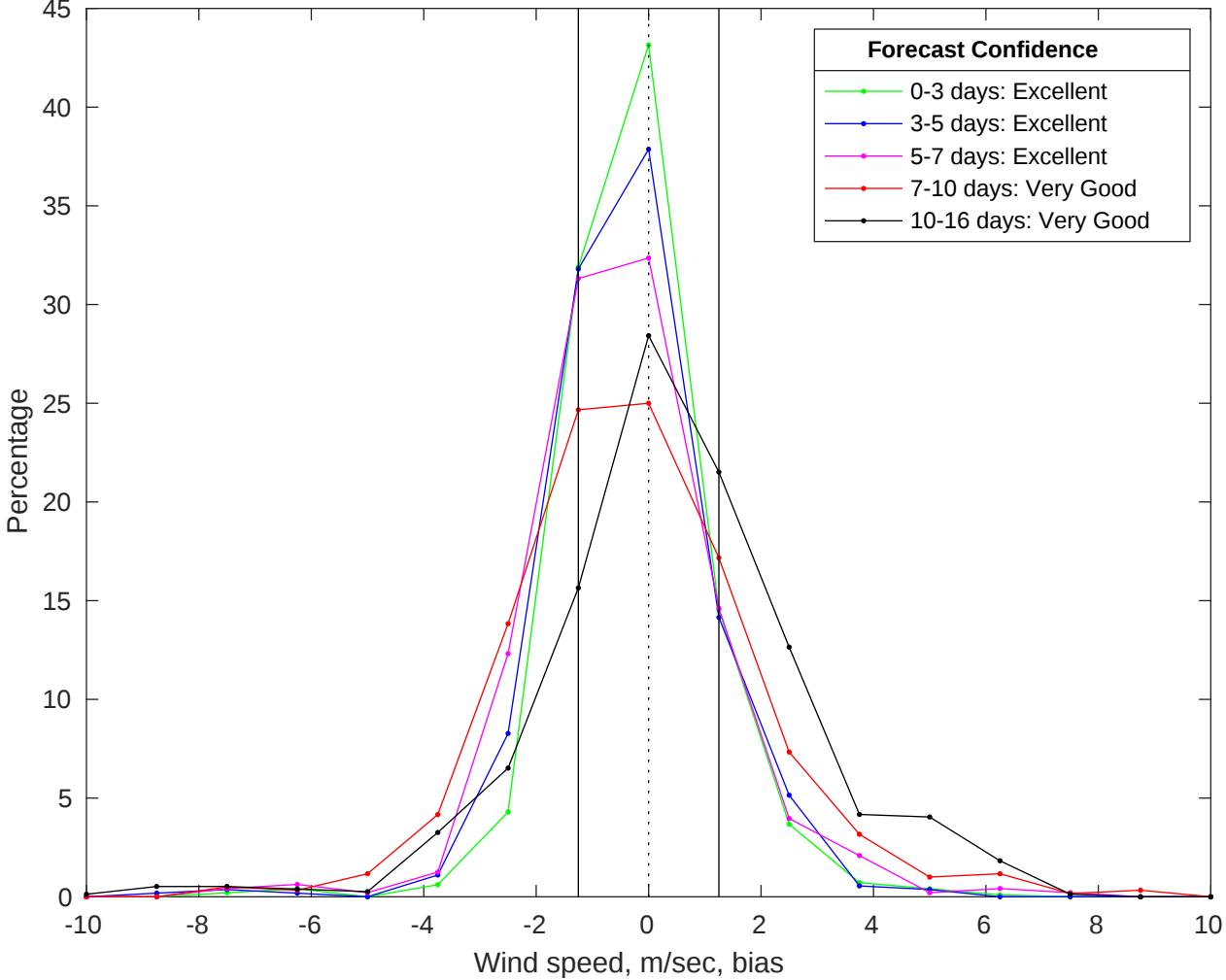
NDBC 42019 vs GFS Winds Bias Histogram: 27-Jul-2025
