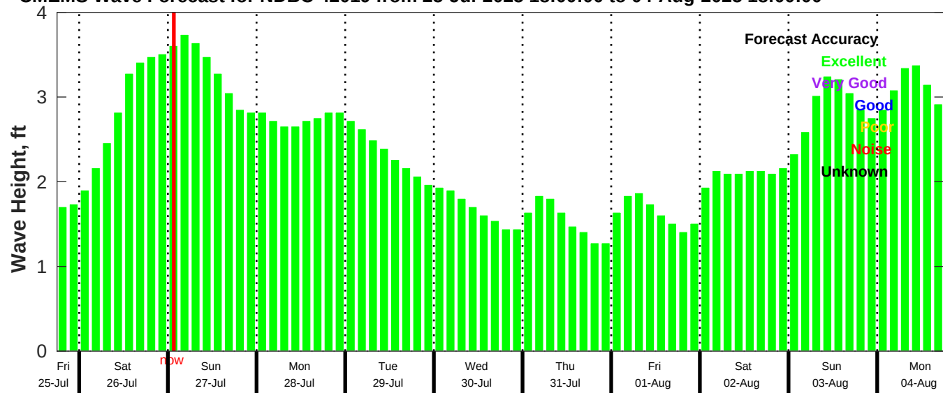
CMEMS Wave Forecast for NDBC 42019 from 25-Jul-2025 18:00:00 to 04-Aug-2025 18:00:00
