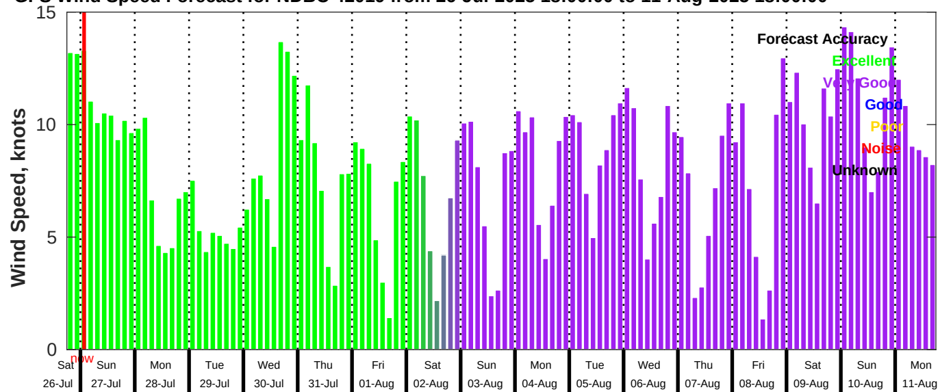
GFS Wind Speed Forecast for NDBC 42019 from 26-Jul-2025 18:00:00 to 11-Aug-2025 18:00:00
