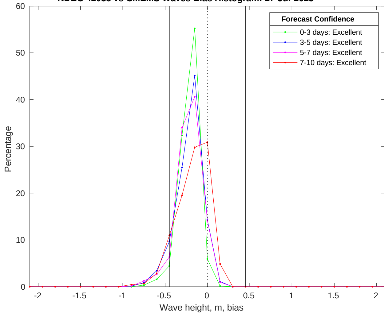
NDBC 42035 vs CMEMS Waves Bias Histogram: 27-Jul-2025
