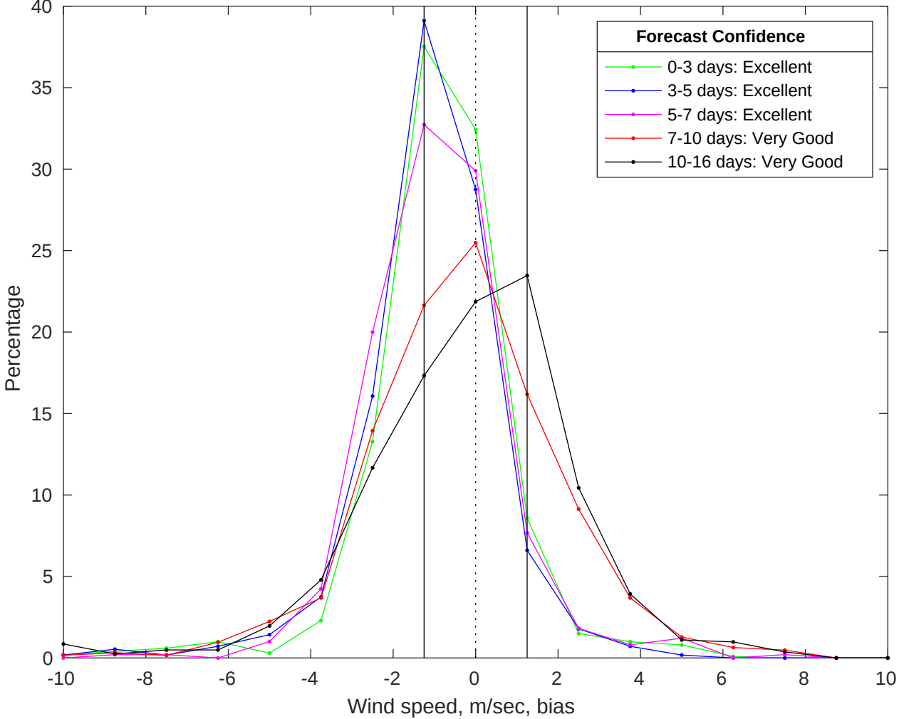
NDBC 42035 vs GFS Winds Bias Histogram: 27-Jul-2025
