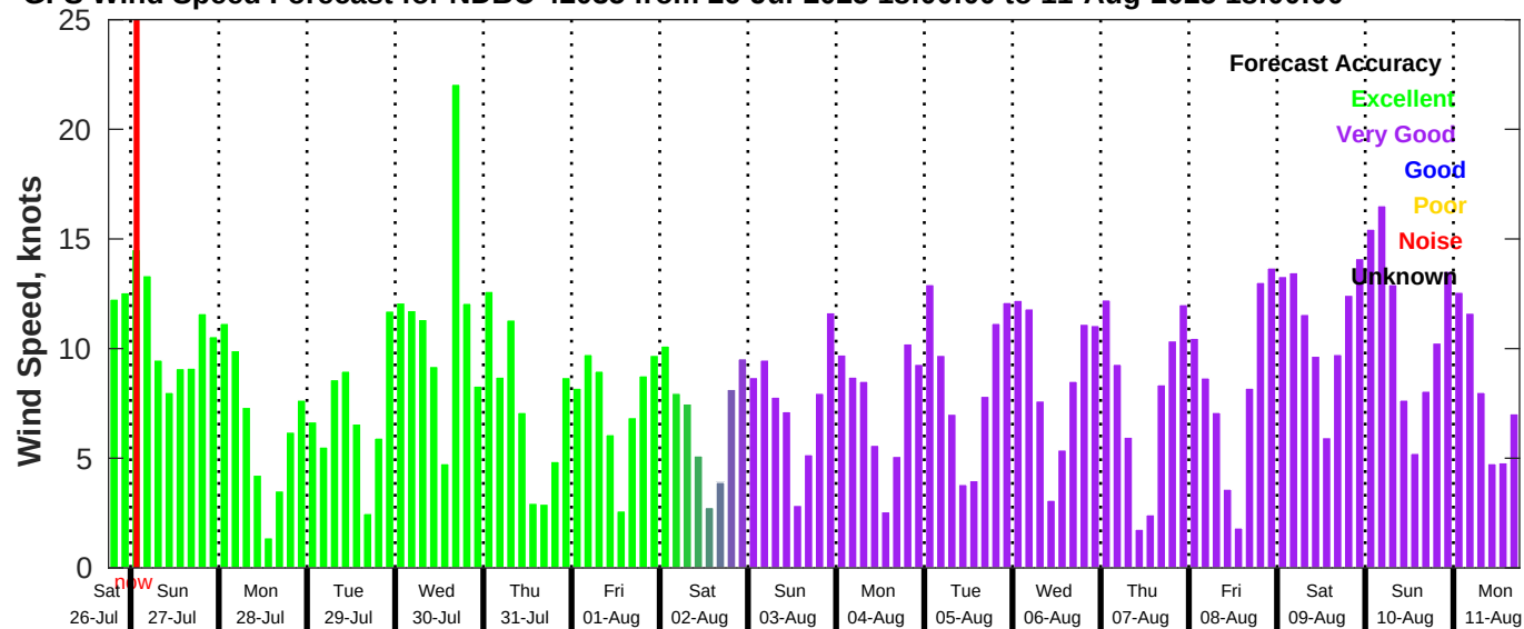
GFS Wind Speed Forecast for NDBC 42035 from 26-Jul-2025 18:00:00 to 11-Aug-2025 18:00:00
