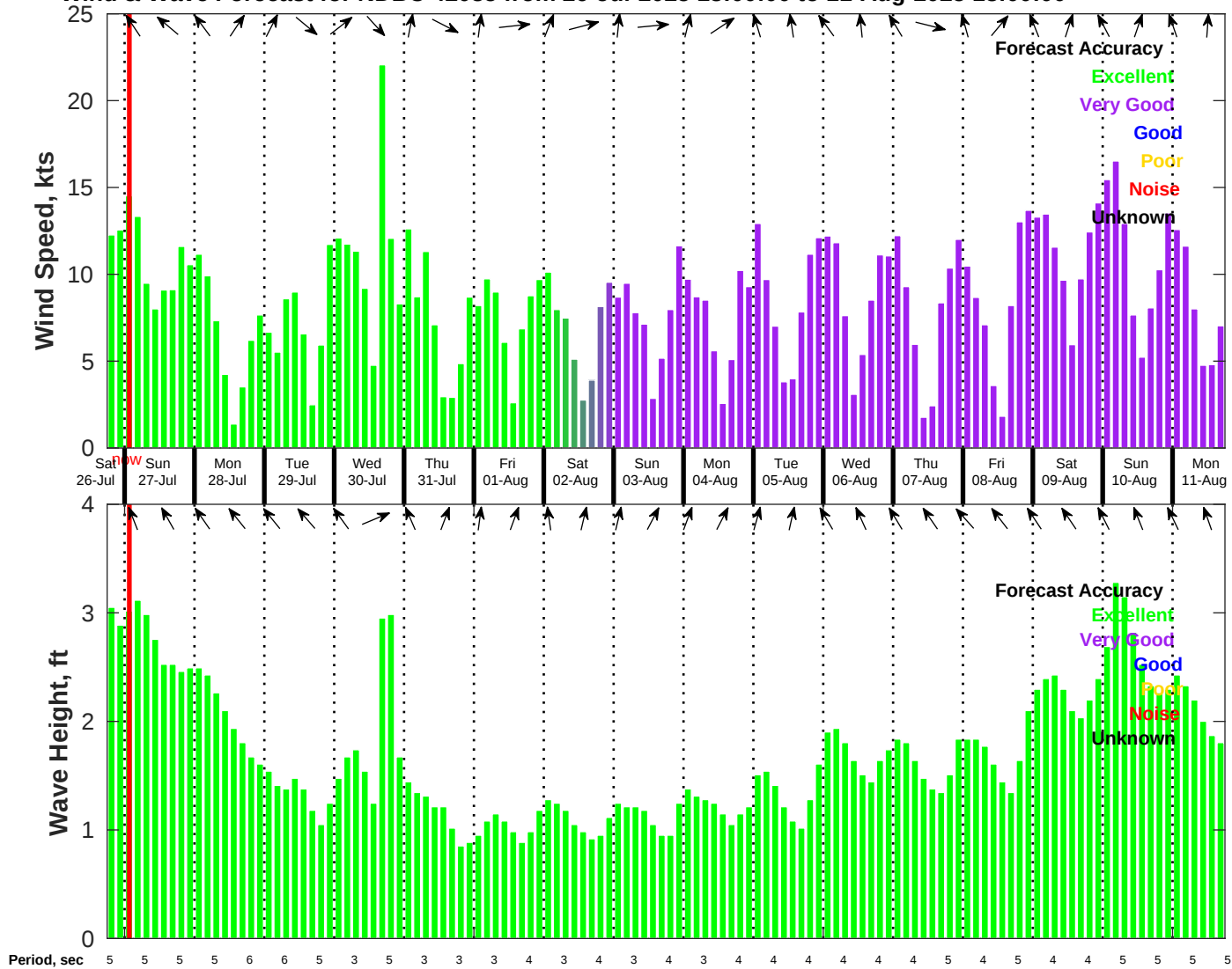
Wind & Wave Forecast for NDBC 42035 from 26-Jul-2025 18:00:00 to 11-Aug-2025 18:00:00
