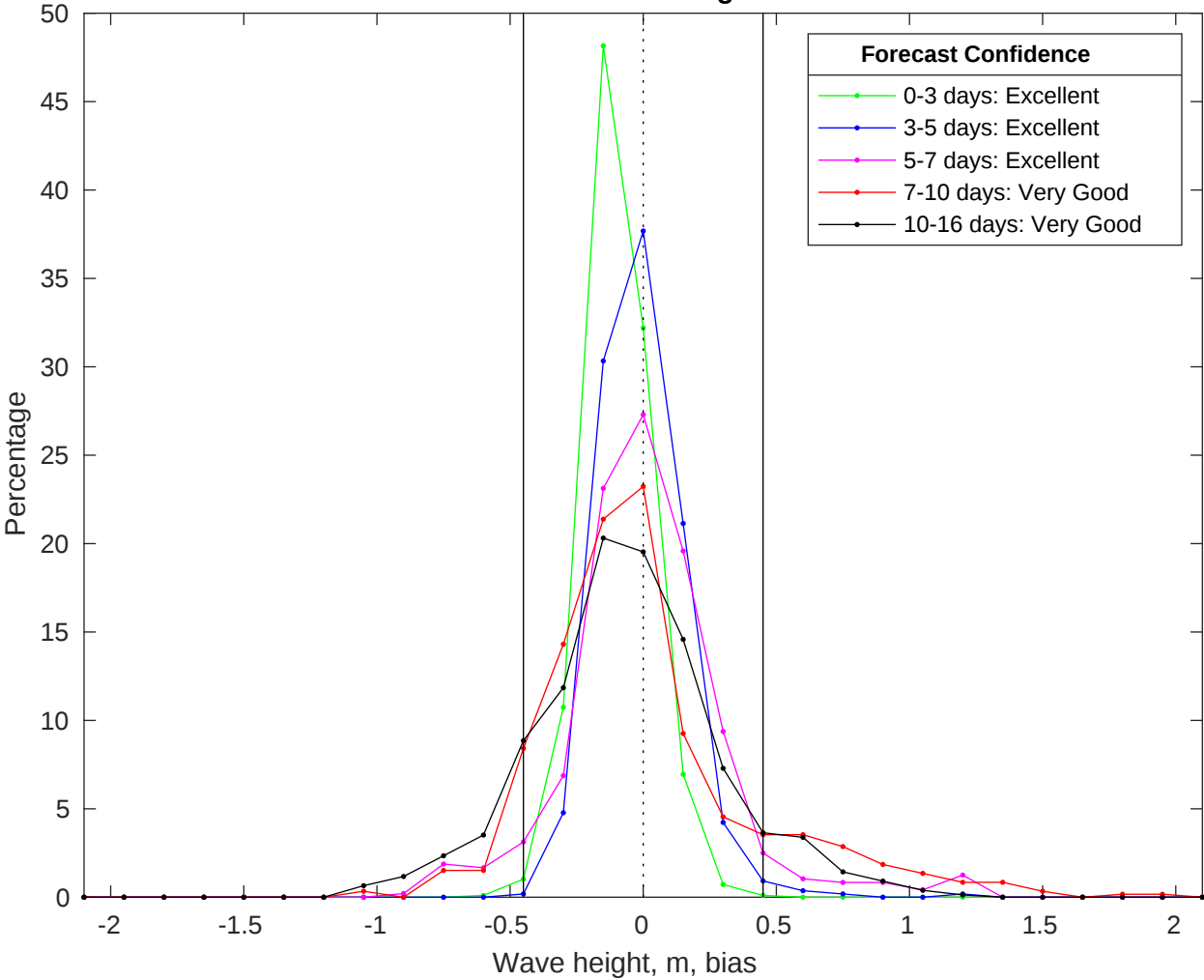
NDBC 42036 vs GFS Waves Bias Histogram: 27-Jul-2025
