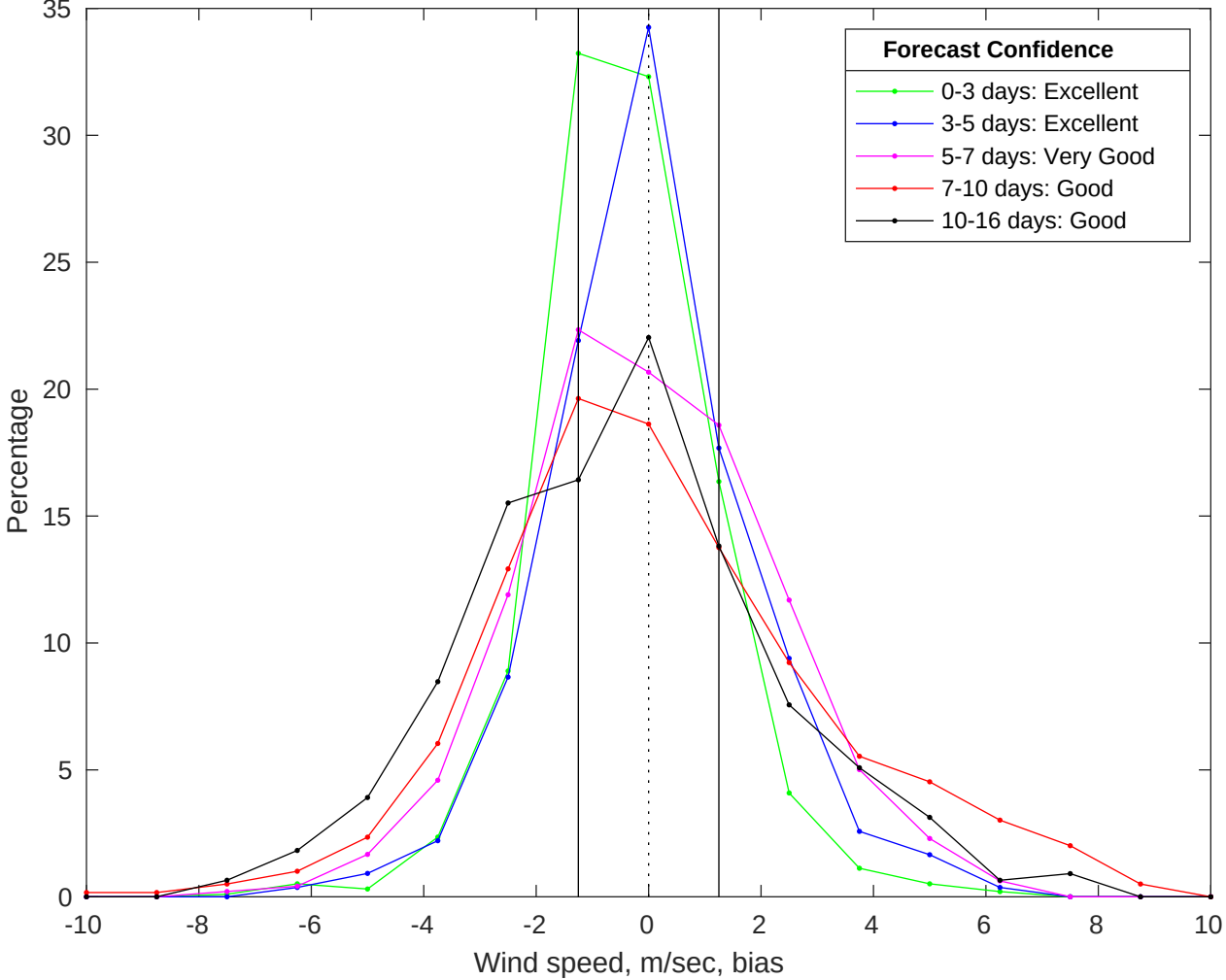
NDBC 42036 vs GFS Winds Bias Histogram: 27-Jul-2025
