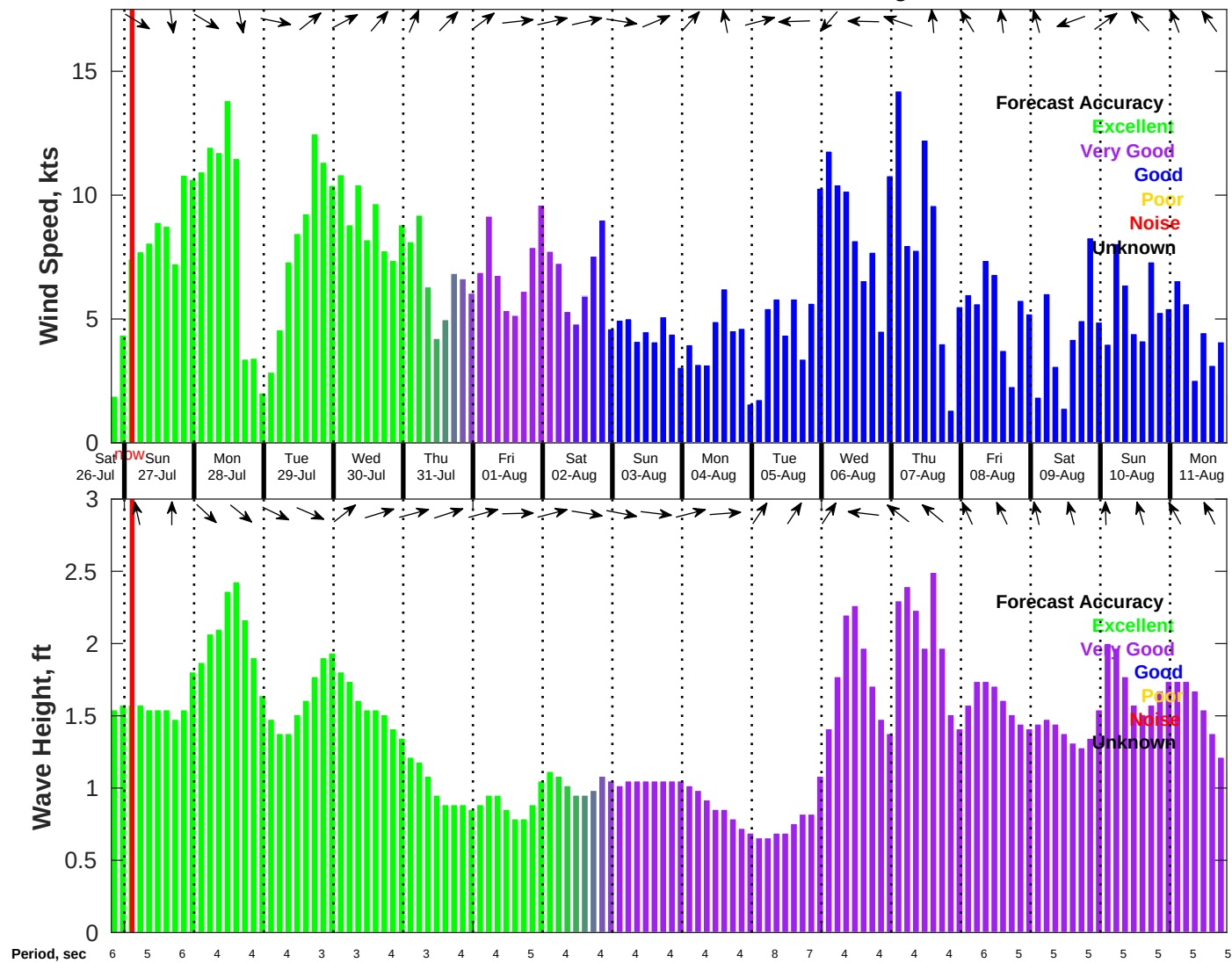
Wind & Wave Forecast for NDBC 42036 from 26-Jul-2025 19:00:00 to 11-Aug-2025 19:00:00
