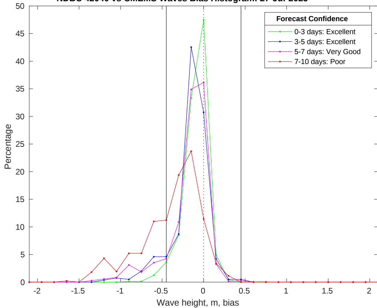
NDBC 42040 vs CMEMS Waves Bias Histogram: 27-Jul-2025
