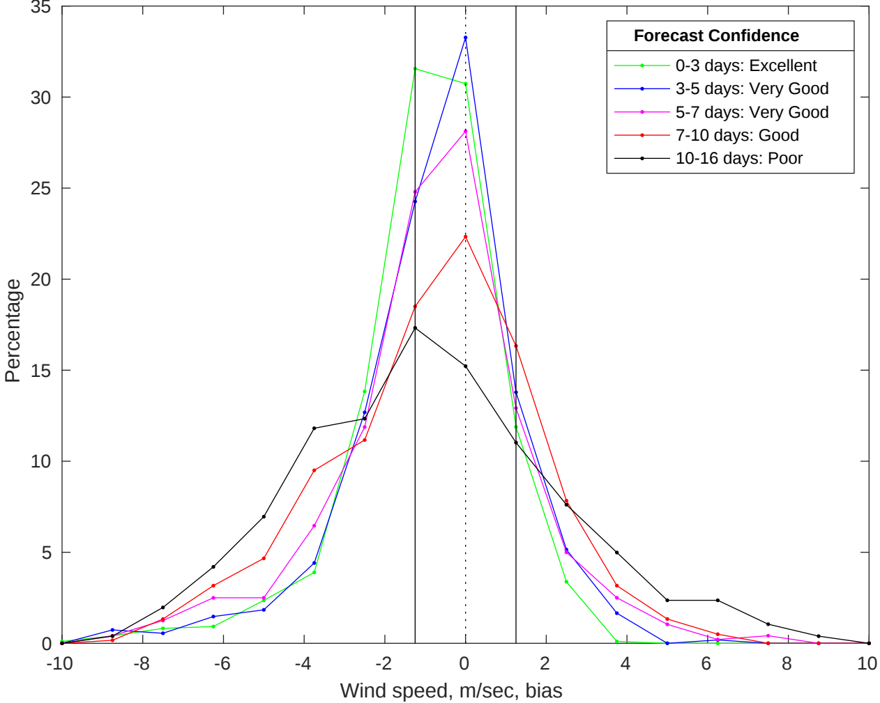
NDBC 42040 vs GFS Winds Bias Histogram: 27-Jul-2025
