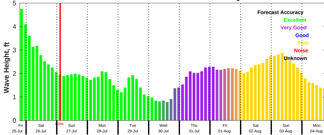
CMEMS Wave Forecast for NDBC 42040 from 25-Jul-2025 19:00:00 to 04-Aug-2025 19:00:00
