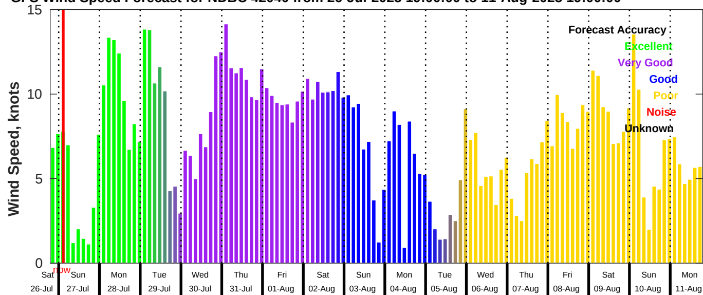
GFS Wind Speed Forecast for NDBC 42040 from 26-Jul-2025 19:00:00 to 11-Aug-2025 19:00:00
