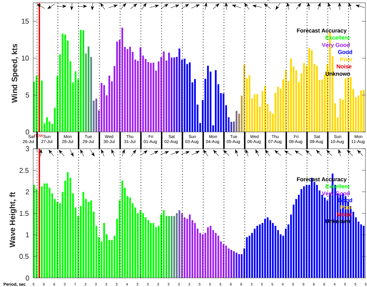
Wind & Wave Forecast for NDBC 42040 from 26-Jul-2025 19:00:00 to 11-Aug-2025 19:00:00
