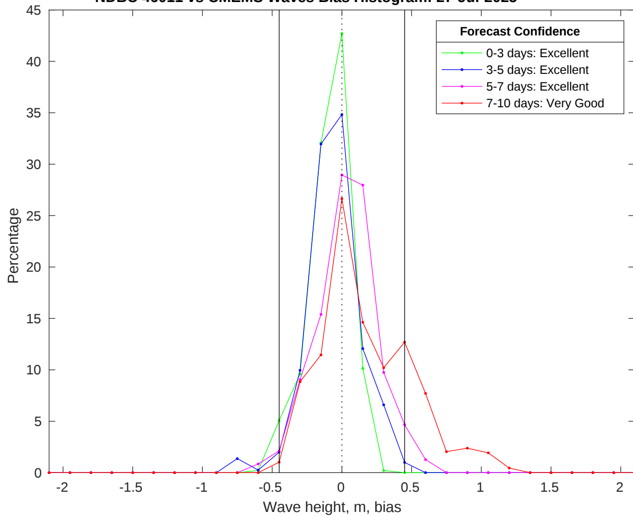
NDBC 46011 vs CMEMS Waves Bias Histogram: 27-Jul-2025
