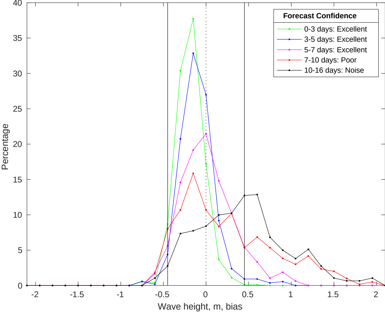
NDBC 46011 vs GFS Waves Bias Histogram: 27-Jul-2025
