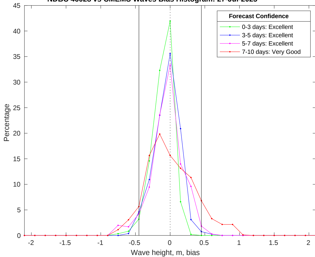
NDBC 46028 vs CMEMS Waves Bias Histogram: 27-Jul-2025
