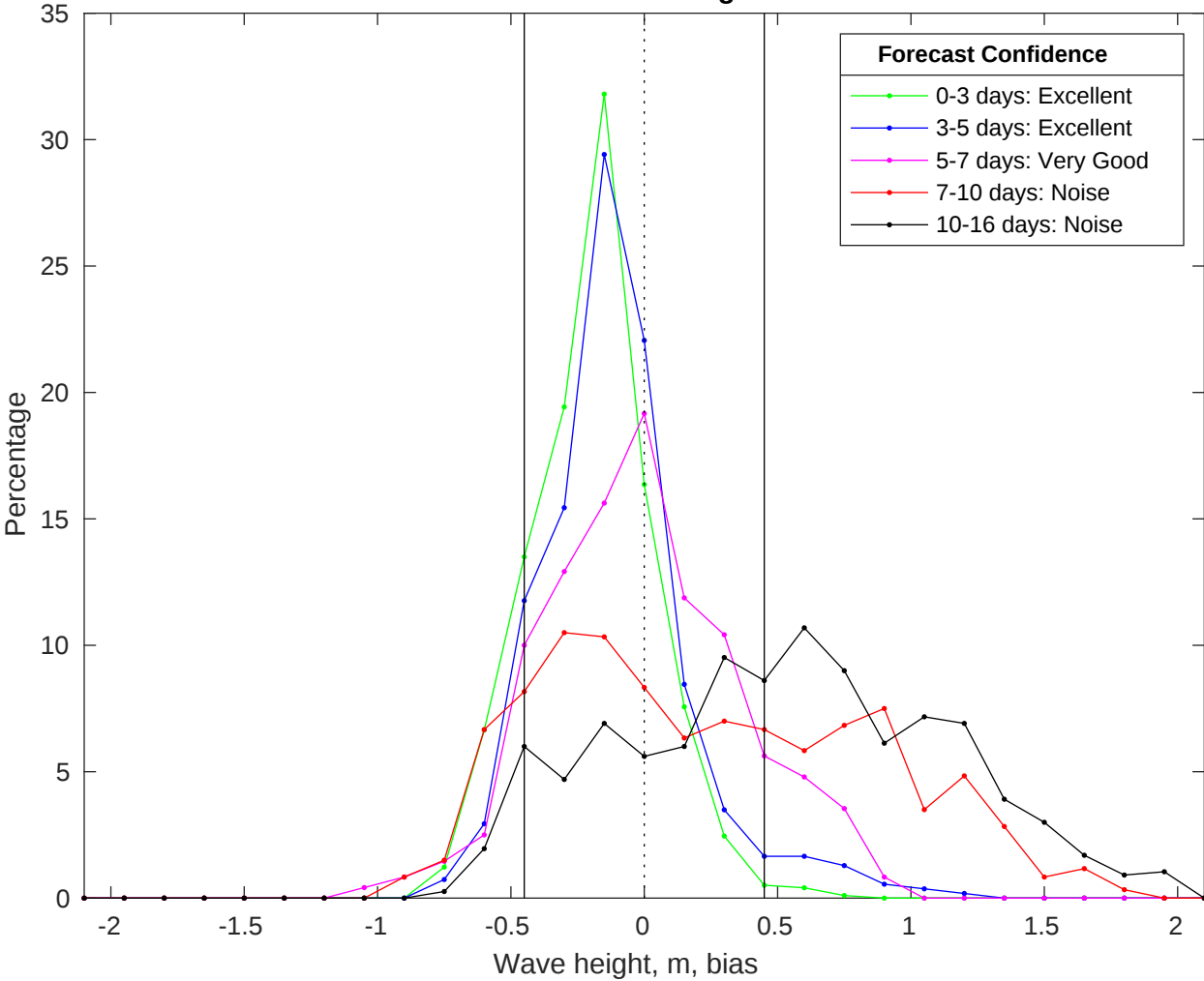
NDBC 46028 vs GFS Waves Bias Histogram: 27-Jul-2025
