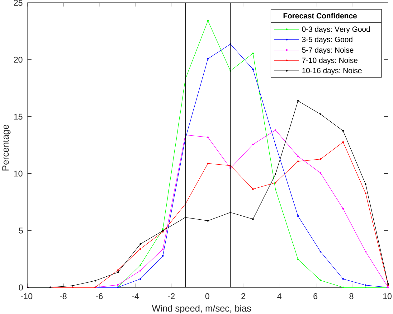
NDBC 46028 vs GFS Winds Bias Histogram: 27-Jul-2025
