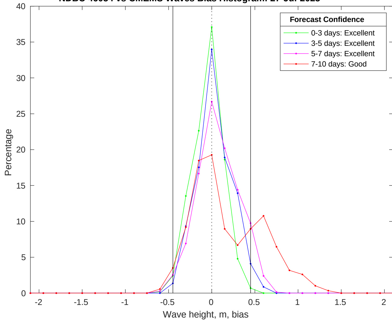
NDBC 46054 vs CMEMS Waves Bias Histogram: 27-Jul-2025
