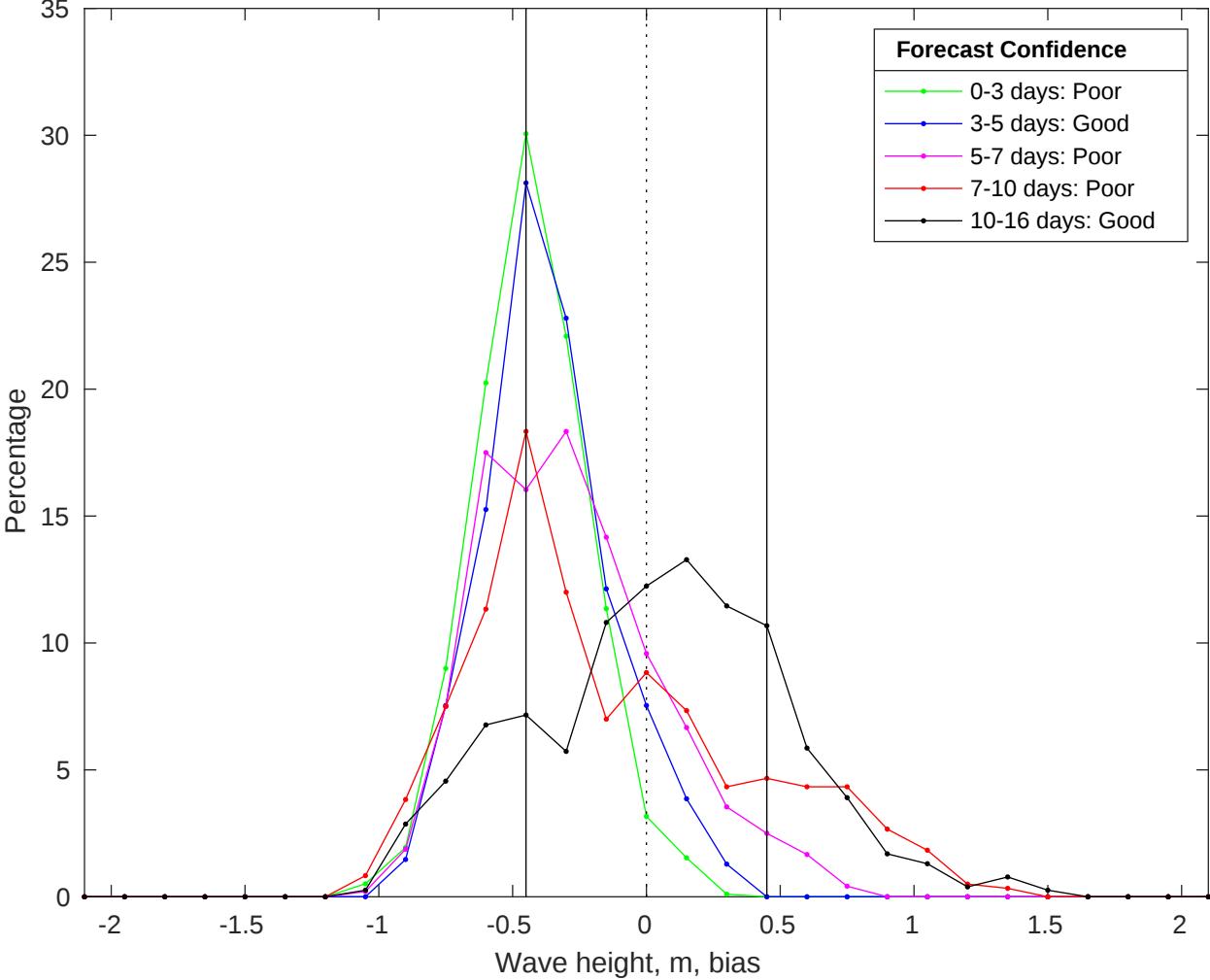
NDBC 46054 vs GFS Waves Bias Histogram: 27-Jul-2025
