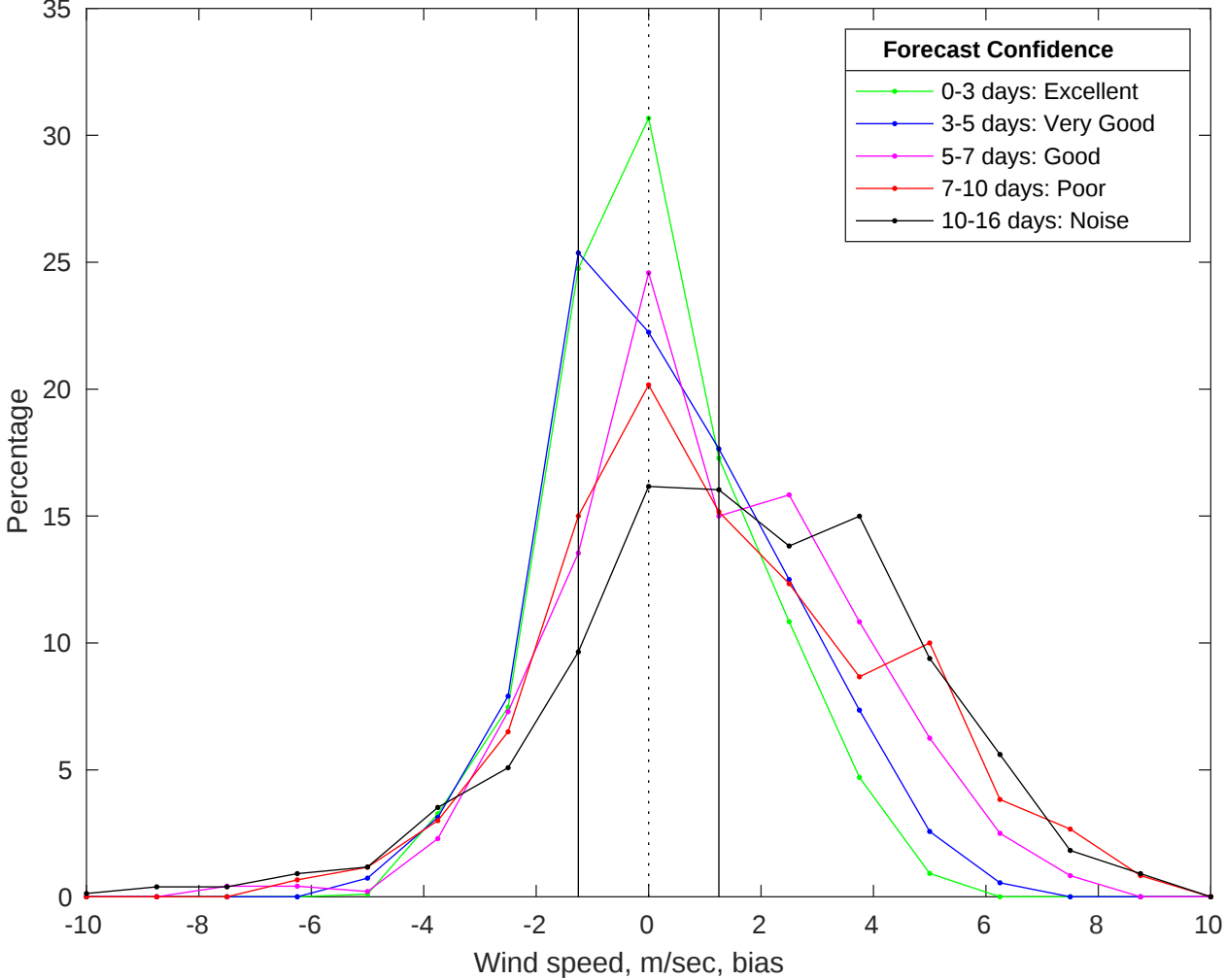
NDBC 46054 vs GFS Winds Bias Histogram: 27-Jul-2025
