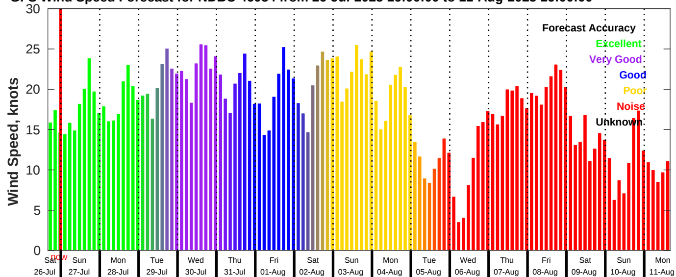
GFS Wind Speed Forecast for NDBC 46054 from 26-Jul-2025 16:00:00 to 11-Aug-2025 16:00:00
