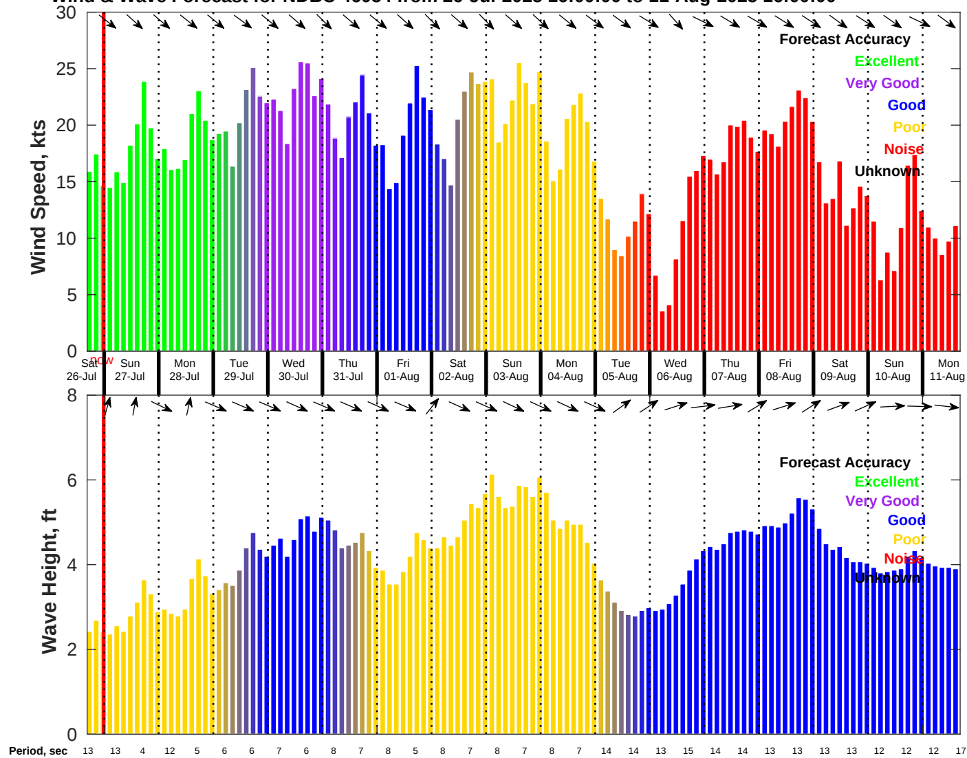
Wind & Wave Forecast for NDBC 46054 from 26-Jul-2025 16:00:00 to 11-Aug-2025 16:00:00
