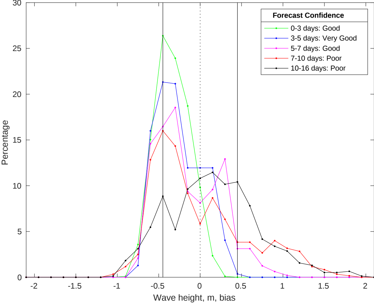
NDBC 46069 vs GFS Waves Bias Histogram: 27-Jul-2025
