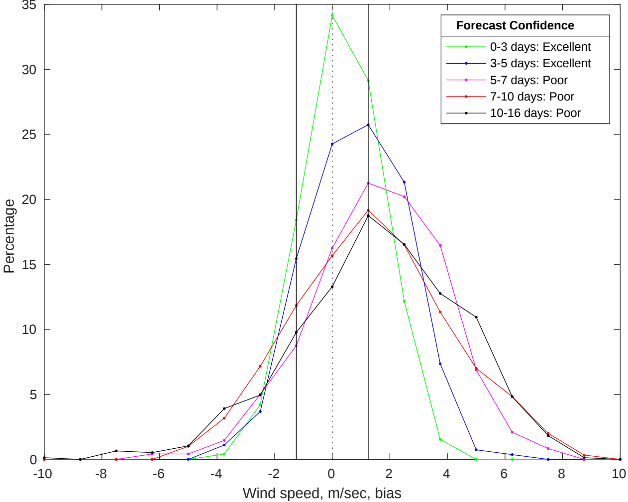
NDBC 46069 vs GFS Winds Bias Histogram: 27-Jul-2025
