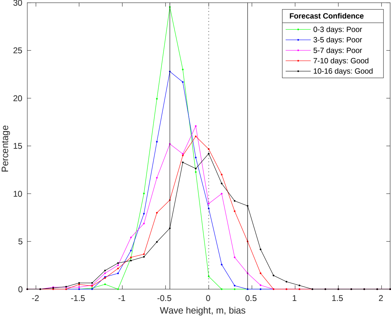
NDBC 51209 vs GFS Waves Bias Histogram: 27-Jul-2025
