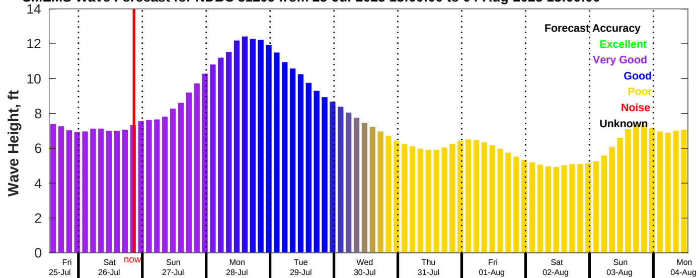
CMEMS Wave Forecast for NDBC 51209 from 25-Jul-2025 13:00:00 to 04-Aug-2025 13:00:00
